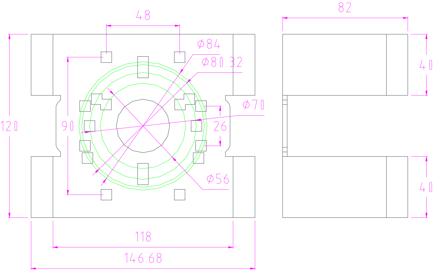
VISTA FRONTAL
